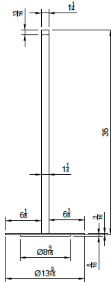
SIDE
